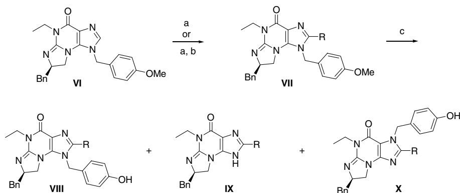
Scheme 2. Synthesis of N-1/N-3/C-2 derivatives. Reagents and conditions: (a) NBS, NCS, or NIS; (b) phenylacetylene, CuI, PdCl 2 (PPh 3 ) 2 ; (c) BBr 3 .
